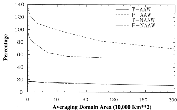
FIG. 12. The percentage ratio rmsd/(amplitude of annual cycle) vs averaging domain area.
