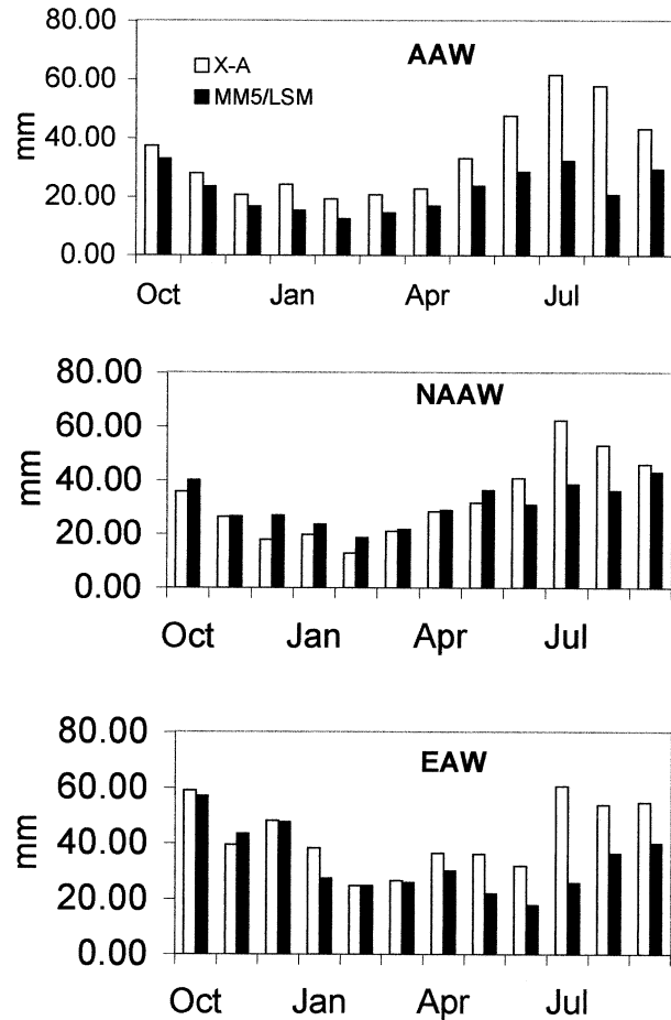
FIG. 10. Annual cycle of monthly accumulated precipitation for each of the continental analysis regions.
