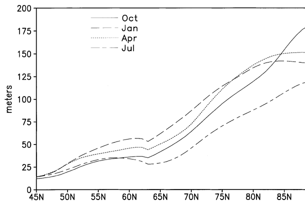
FIG. 4. Root-mean-square difference in 500-hPa geopotential height between simulation and NCEP–NCAR reanalysis, as a function of latitude for 4 months of the simulation period. Curves are monthly averages of daily rmsd.
