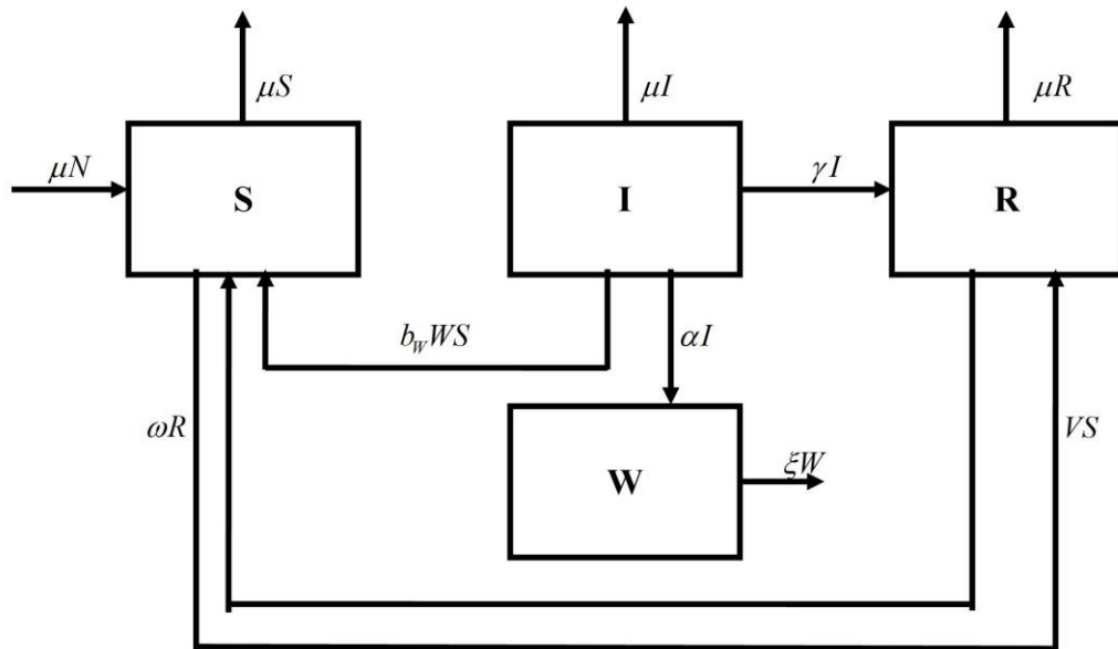
Figure 1 Flow diagram of the SIWR model.
