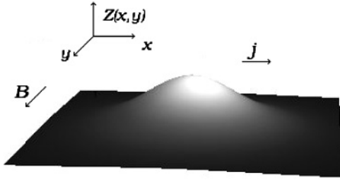
FIG. 1. Interface between normal and superconducting regions in a type-I superconductor, pinned by a planar defect in the XY plane. Transport current parallel to the interface controls the energy barrier. Depinning of the interface occurs through quantum nucleation of a critical bump described by the instanton of the equations of motion in 2 + 1 dimensions.
