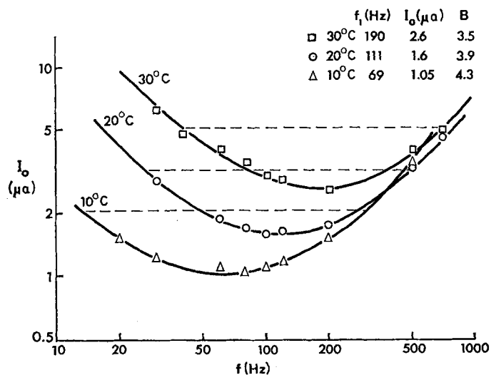
FIGURE 6. Strength-frequency (resonance) curve of space-clamped squid axon, stimulated by AC sinusoidal current at 10°, 20°, and 30°C, respectively. Threshold current in microamperes vs. frequency (Hz), both on log scales. Note that the effect of temperature is much greater at low frequencies than in the high frequency (capacitive) region. Note also that both optimum frequency and threshold current increase with increasing temperature, while the width index, B, decreases. A dashed line is drawn across each curve at a current intensity twice that of the threshold current at the optimum frequency for calculation of B, the width index.
