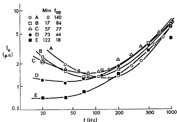
FIGURE 2. Effect of deterioration upon resonance curve of space-clamped squid axon stimulated by sinusoidal AC current. Threshold current, I_o , in microamperes vs. frequency (Hz) both on log scales. Curves recorded at times indicated. All points on same axon at 10^\circ\text{C} in artificial seawater. See text for discussion.
