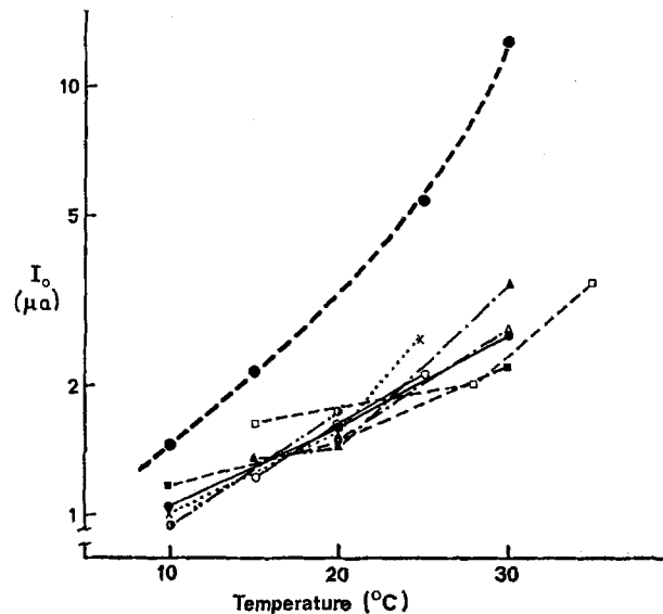
FIGURE 7. Effect of temperature on threshold current, I_o , required at optimum frequency for both real and computed axons. Current in microamperes on log scale vs. temperature in ^{\circ}C on linear scale. Composite of runs on eight real axons displaced up or down by an average of 17.5% for best fit. Theoretical run not displaced. Units on ordinate refer to computed axon only. Note that the computed axon is more temperature-dependent than the real axons. See text for further discussion.
