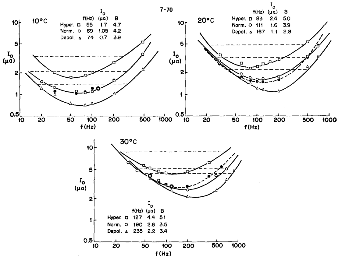
FIGURE 9. Effect of 15 mv depolarizing and hyperpolarizing currents on resonance curves of real space-clamped squid axons at 10°, 20°, and 30°C. Threshold current in microamperes vs. frequency (Hz) both on log scales. All points taken on same axon. Note excellent recovery (solid circles) in each case. Typical results. See text for discussion of results.
