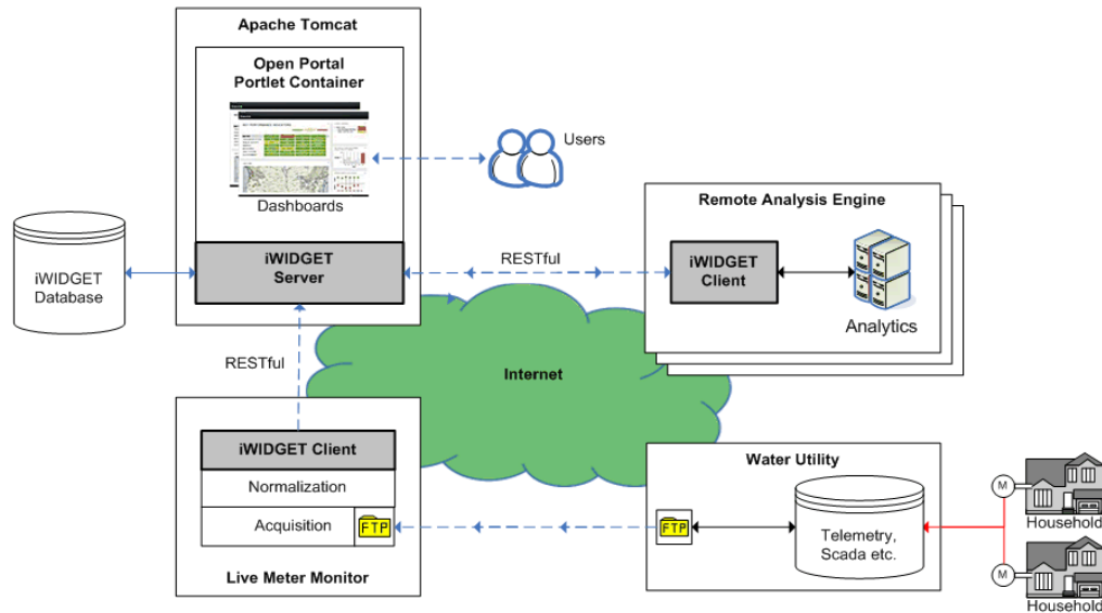
Figure 1. iWIDGET Distributed Architecture
