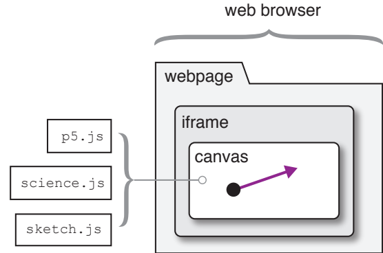
FIG. 1. The schematic layout of a sim as embedded element in a webpage. The sim, where the code is stored in the sketch.js file, draws to the canvas using the other libraries shown.
