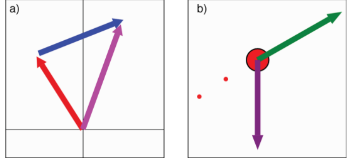
FIG. 4. a) Vector addition sim. Users can drag the red and blue vectors and the purple arrow updates to portray the vector sum. b) A KineticMass() object with velocity and acceleration vectors added.
