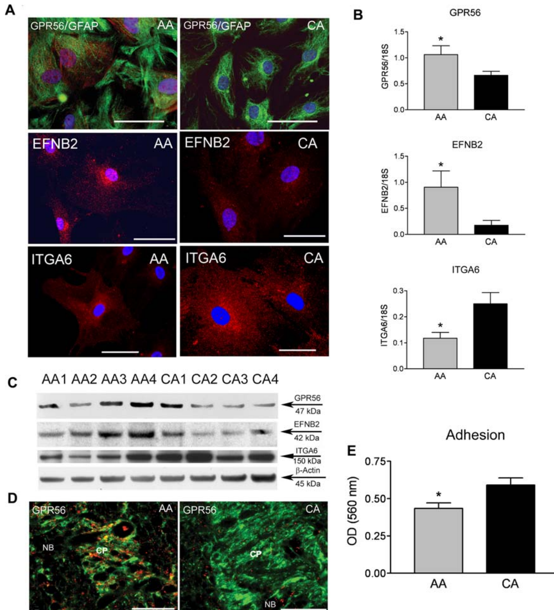
Figure 3. AA astrocytes exhibit decreased cell adhesion compared to CA astrocytes. A. Cellular localization of G protein-coupled receptor 56 (GPR56), ephrin-B2 (EFNB2) and integrin \alpha 6 (ITGA6) in primary cultures of ONH astrocytes. Nuclei stained with DAPI (blue). Magnification bar: 25 \mu m. Upper: Double immunofluorescence for GFAP (green), an intermediate filament characteristic of astrocytes and GPR56 (red). Note granular staining for GPR56 (red) is more abundant in the cytoplasm of AA astrocytes compared to CA astrocytes. Middle: Immunofluorescence showed that EFNB2 is more abundant in the cytoplasm of AA astrocytes compared to CA astrocytes. Lower: Immunofluorescence showed that Integrin \alpha 6 is less abundant in the cytoplasm of AA astrocytes compared to CA astrocytes. B. Confirmation of three differentially expressed adhesion genes by qRT-PCR in human normal ONH astrocytes: GPR56, EFNB2 and ITGA6. Genes were normalized to 18S. Graphical representation of the relative mRNA levels in AA and CA astrocytes (n=8, respectively, *indicates p < 0.05 in two-tailed t-test). C. Representative Western blots of astrocyte cell lysates with GPR56, EFNB2 and ITGA6 antibodies. \beta -actin was used as a loading control. Note that AA1-4 donors express more GPR56 and EFNB2, less ITGA6 than CA1-4 donors. D. Representative immunohistochemistry showed more abundant granular staining of GPR56 (red) in astrocytes in the lamina cribrosa from AA donors compared to CA donors. Note that GPR56 is also localized in astrocyte processes in the nerve bundles (NB). CP: cribriform plates, Magnification bar: 25 \mu m. E. AA astrocytes adhered to collagen IV 26.5% less than CA astrocytes did (* indicates p < 0.05 in two-tailed t-test). Values represent mean optical density (OD) \pm standard deviation of triplicate experiments using primary astrocyte cultures of four AA donors and six CA donors. doi:10.1371/journal.pone.0002847.g003
