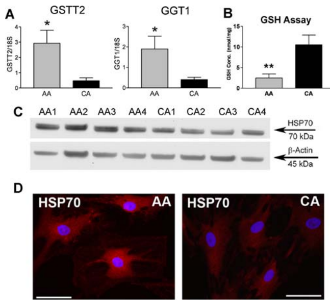
Figure 6. Upregulation of glutathione (GSH) metabolic enzymes in AA astrocytes. A. Confirmation of two differentially expressed glutathione metabolic enzyme genes by qRT-PCR in human normal ONH astrocytes: glutathione S-transferase theta 2 (GSTT2) and gamma-glutamyltransferase 1 (GGT1). Genes were normalized to 18S. Graphical representation of the relative mRNA levels in AA and CA astrocytes (n = 8, respectively, * indicate p < 0.05 in two-tailed t-test). B. AA astrocytes have significantly lower level of intracellular GSH in vitro , compared to CA astrocytes (n = 10, ** indicated p < 0.01 in two-tailed t-test). GSH content is normalized by the amount of the protein. C. Representative Western blots of astrocyte cell lysates with heat shock 70 kDa protein (HSP70) antibody. \beta -actin was used as a loading control. HSP70 levels are higher in AA astrocytes compared to CA astrocytes. D. Immunofluorescent staining for HSP70 shows that AA astrocytes exhibit more abundant intracellular HSP70 staining compared to CA astrocytes. Magnification bar: 25 \mu m. doi:10.1371/journal.pone.0002847.g006
