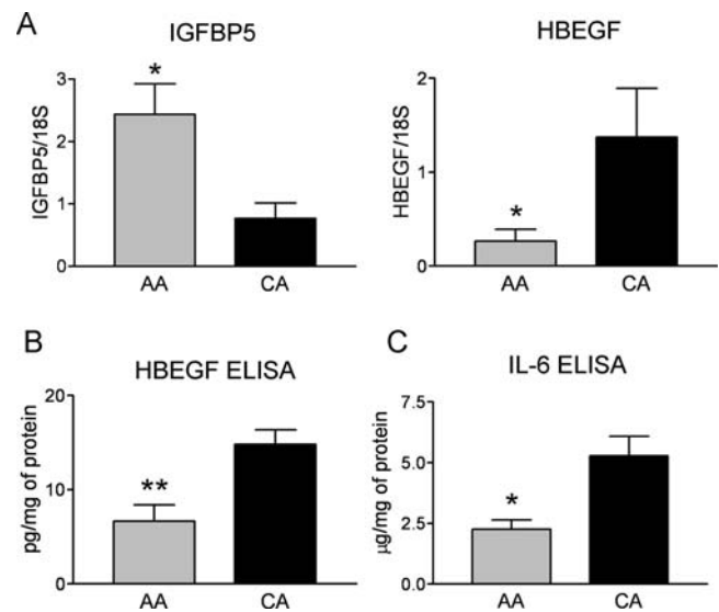
Figure 7. Differential expression of growth factors and cytokines in AA astrocytes. A. Confirmation of two differentially expressed growth factor genes by qRT-PCR in human normal ONH astrocytes: insulin-like growth factor binding protein 5 (IGFBP5) and heparin-binding EGF-like growth factor (HBEGF). Genes were normalized to 18S. Graphical representation of the relative mRNA levels in normal AA and CA astrocytes (n = 8, respectively, two-tailed t-test was used. * indicate p < 0.05 ). B., C. Seven CA samples and six AA samples were used in ELISA experiment. B. The total amount of secreted and intracellular HBEGF is significantly lower in AA astrocytes compared to CA astrocytes (** indicated p < 0.01 in two-tailed t-test) C. The level of secreted IL-6 is significantly lower in AA astrocytes compared to CA astrocytes (* indicated p < 0.05 in two-tailed t-test). doi:10.1371/journal.pone.0002847.g007
