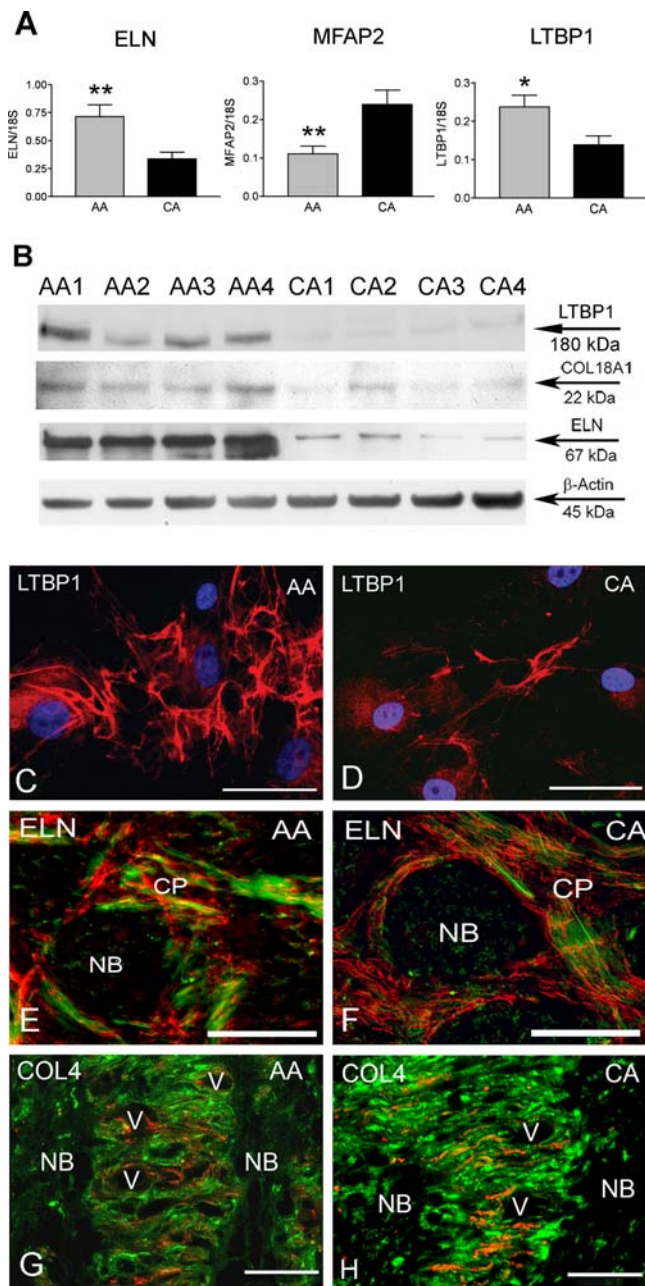
Figure 5. Differential expression of genes associated with the extracellular matrix (ECM) in AA astrocytes compared to CA astrocytes. A. Confirmation of three differentially expressed adhesion genes by qRT-PCR in human normal ONH astrocytes: Elastin (ELN), microfibrillar-associated protein 2 (MFAP2) and latent transforming growth factor beta binding protein 1 (LTBP1). Genes were normalized to 18S. Graphical representation of the relative mRNA levels in normal AA and CA astrocytes ( n=8 , respectively, two-tailed t-test was used. ** indicates p<0.01 and * indicate p<0.05 ). B. Representative Western blots of astrocyte cell lysates with LTBP1, ELN and collagen type XVIII antibodies. \beta -actin was used as a loading control. Note that AA1-4 donors express more LTBP1, ELN and collagen type XVIII than CA1-4 donors. C, D. Immunocytochemistry of LTBP1 in AA and CA astrocytes. LTBP1 (red) is more abundant in the cytoplasm and extracellular space in AA astrocytes compared with CA astrocytes. Nuclei stained with DAPI (blue). Magnification Bar: 25 \mu m. E, F. Double immunostaining of ELN (red) and GFAP (green) in representative cross sectional of the ONH tissue in AA and CA donors. ELN is located in the cribriform plates and not in the nerve bundles. Astrocytes cell bodies are located in the cribriform plates (CP) and extend processes into the nerve bundle (NB).
