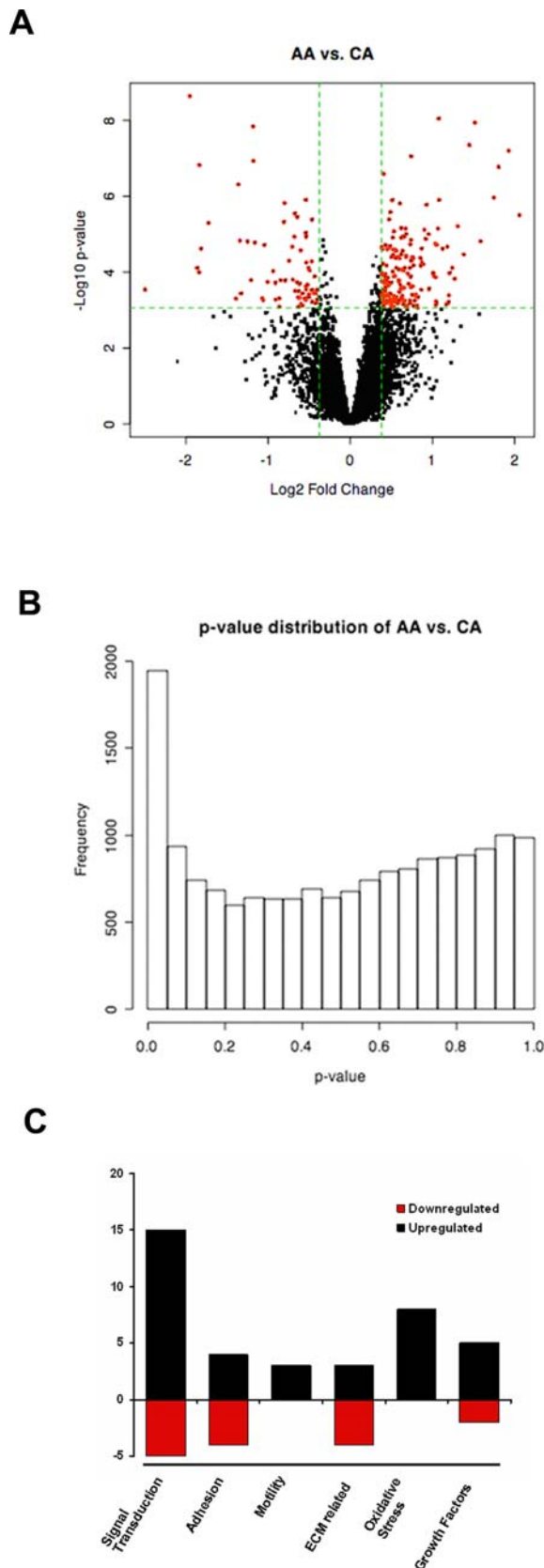
Figure 1. Differential gene expression in primary cultures of ONH astrocytes from age-matched normal donors (12 AA and 12 CA). A. Volcano plot indicates the size of biological effect (fold change) versus the statistical significance of the result (statistical p-
