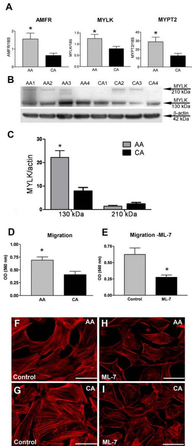
Figure 4. AA astrocytes exhibit increased migration compared to CA astrocytes. A. Confirmation of three differentially expressed motility genes by qRT-PCR in human normal ONH astrocytes: autocrine motility factor receptor (AMFR), myosin light chain kinase (MYLK) and myosin phosphatase target subunit 2 (MYPT2). Genes were normalized to 18S. Graphical representation of the relative mRNA levels in AA and CA astrocytes (n=8, respectively, * indicates p<0.05 in two-tailed t-test). B. Representative Western blots of astrocyte cell lysates with MYLK antibody. β-actin was used as a loading control. Note that AA1-4 donors express more MYLK 130 kDa than CA1-4 donors. No difference
