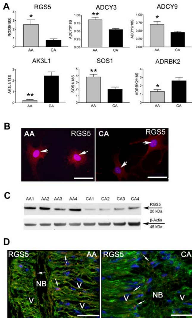
Figure 2. Signal transduction pathways in AA astrocytes compared to CA astrocytes. A. Confirmation of six differentially expressed signaling genes by qRT-PCR in human normal ONH astrocytes: RGS5, ADCY3, ADCY9, AK3L1, SOS1 and ADRBK2. Genes were normalized to 18S. Graphical representation of the relative mRNA levels in normal AA and CA astrocytes ( n=8 , respectively, two-tailed t test was used. ** indicates p<0.01 and * indicates p<0.05 ). B. Cellular localization of the Regulator of G protein signaling 5 (RGS5) in primary cultures of ONH astrocytes. Immunofluorescent staining of RGS5 (red) demonstrated higher levels of RGS5 protein in AA astrocytes, compared to CA astrocytes. Nuclei stained with DAPI (blue). Note that RGS5 localizes to the cytoplasm and in the nucleus of astrocytes (arrows). Magnification bar: 25 \mu m. C. Representative Western blots of astrocyte cell lysates with human RGS5 antibody and \beta -actin used as a loading control. Note that AA1-4 normal donors express more RGS5 than CA1-4 donors. D. Representative double immunofluorescent staining of RGS5 (red) astrocyte marker GFAP (green) in sections of human ONH from an AA donor (71 year-old male) and a CA donor (75 year-old male). Nuclei stained with DAPI (blue). Note strong granular staining of RGS5 in astrocytes (arrows) in the cribriform plates in the lamina cribrosa. Fewer astrocytes stain for RGS5 in the lamina cribrosa of a CA donor. V: blood vessel, NB: nerve bundle, Magnification bar 55 \mu m. doi:10.1371/journal.pone.0002847.g002
