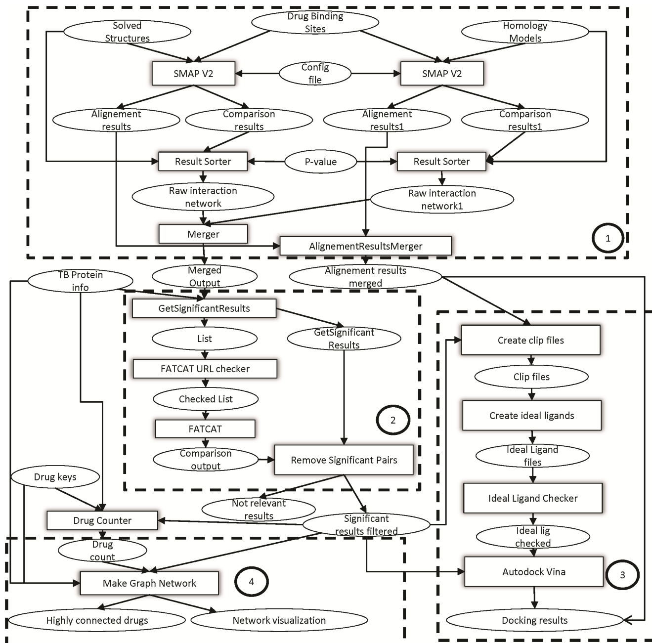
Figure 2. The reproduced TB Drugome workflow with the different subsections highlighted. (1) Comparison of ligand binding sites using SMAP; (2) protein structure comparison using FATCAT; (3) docking using Autodock Vina; and (4) graph network creation (visualization). We focus on the reproducibility of sections 1-3 here. doi:10.1371/journal.pone.0080278.g002
