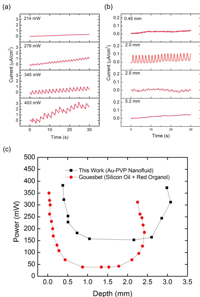
FIG. 2. (a) Plot of the change in the electrical oscillations as a function of the laser-beam intensity. The distance of the laser beam to the meniscus is kept constant. (b) Plot of the change in the electrical oscillations as a function of depth. The laser-beam intensity is kept constant at 440 mW, while oscillations in the measured current and far-field beam profiles are observed. (c) Phase diagram of the primary dynamics of the electrical oscillation in the plane of power and distance of the laser from the free surface for this work and that of Gouesbet [5]. Below the solid line, electrical or optical oscillations are not observed. At most points on this phase diagram above the solid line, the measured currents are nonlinear.
