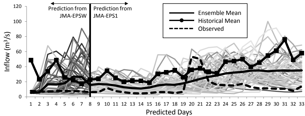
Figure 2. Example of ensemble inflow prediction results (Predicted on 31 st , May, 2007)
