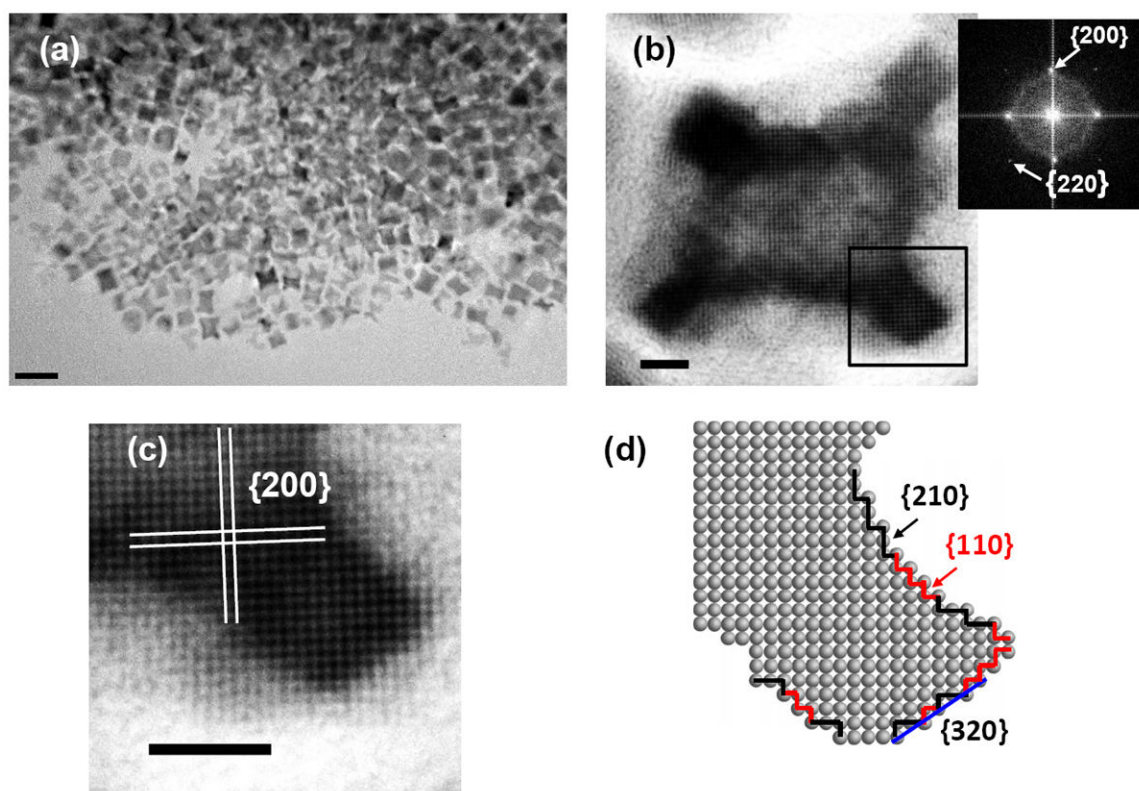
Figure 3. Structural analysis of Pd nanoconcave crystals
