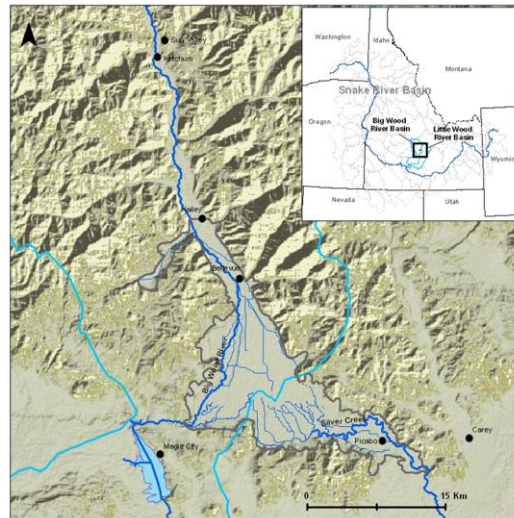
Figure 4. The location and topography of the Big Wood River and Silver Creek.
