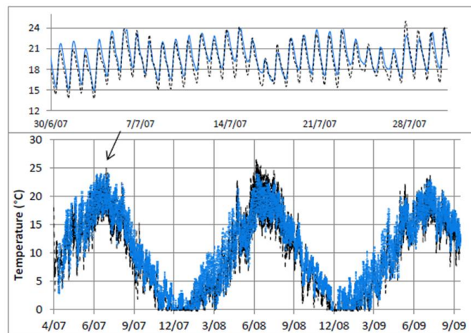
Figure 5. The simulated and observed river temperatures for a single station in Silver Creek.
