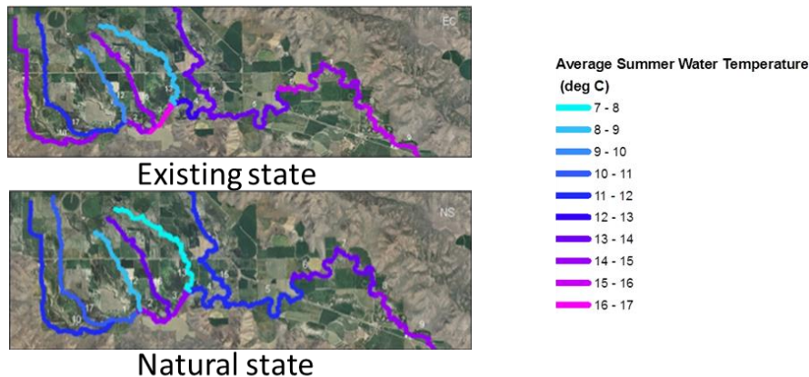
Figure 6. Comparison of the simulated existing and natural state in terms of average daily summer water temperature.
