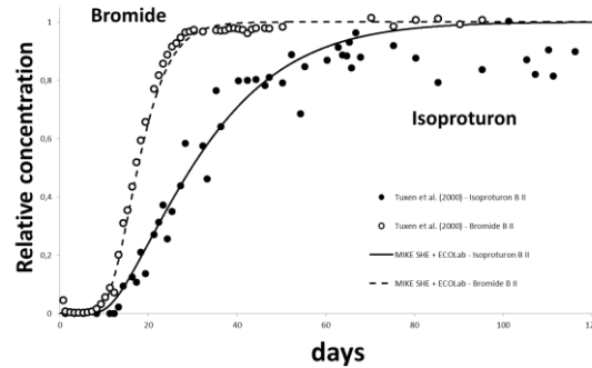
Figure 1. Comparison of the breakthrough curves simulated with MIKE SHE-ECOLAB and the experimental results of Tuxen et al. [13] for bromide and the pesticide isoproturon.
