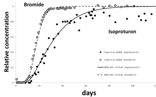
Figure 1. Comparison of the breakthrough curves simulated with MIKE SHE-ECOLAB and the experimental results of Tuxen et al. [13] for bromide and the pesticide isoproturon.
