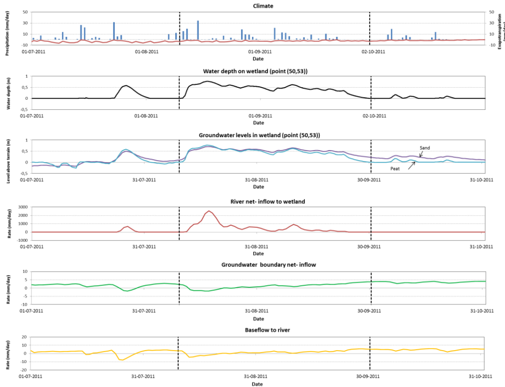
Figure 3. Selected components of the wetland water balance during the flood event in August 2011 (the flood period is marked with dashed black lines).
