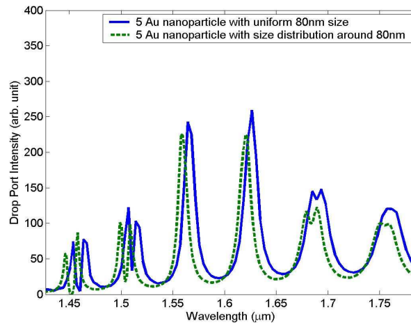
Fig. 4. The Drop port intensity with Au nanoparticle size distribution, 5 Au nanoparticles with uniform 80nm in diameter (solid line) and 5 Au nanoparticles with random size distribution around 80nm in size.
