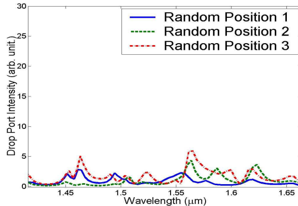
Fig. 3. The Drop port intensity with three random positions of 30 Au nanoparticles with 80nm in size.
