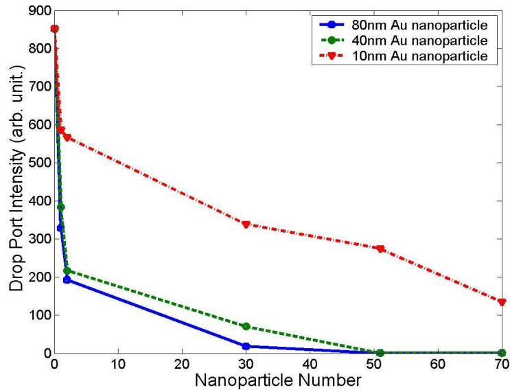
Fig. 5. The Drop intensity vs. nanoparticle number for different size of Au nanoparticles.
