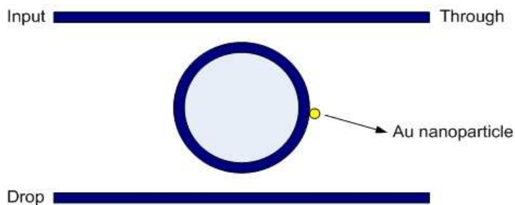
Fig. 1. The on-chip four port micro ring resonator configuration. The core of the micro ring resonator and the two bus waveguides is Si ( n = 3.48 ), with bottom cladding \text{SiO}_2 ( n = 1.45 ) and air cladding on top. The waveguide width is 200nm and satisfies the single mode condition. The Au nanoparticle is adsorbed on the micro ring resonator.
