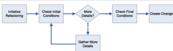
Figure 2: Refactoring Life-Cycle
