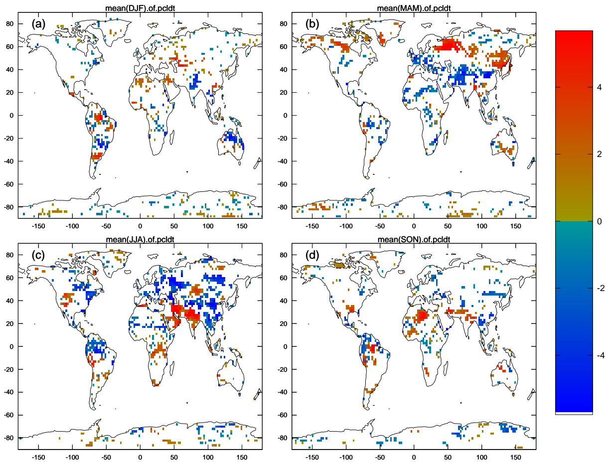
Fig. 4. Change in seasonal cloud cover (%) induced by soil moisture feedback (DYNA minus CLIM run). (a) DJF, (b) MAM, (c) JJA, (d) SON.
