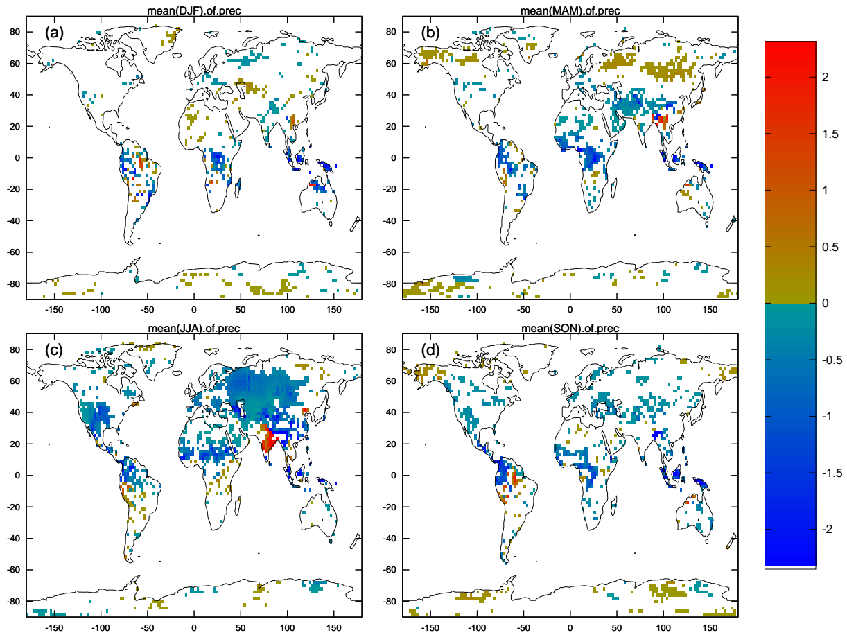
Fig. 2. Change in seasonal precipitation (mm/day) induced by soil moisture feedback (DYNA minus CLIM run). (a) DJF, (b) MAM, (c) JJA, (d) SON.
