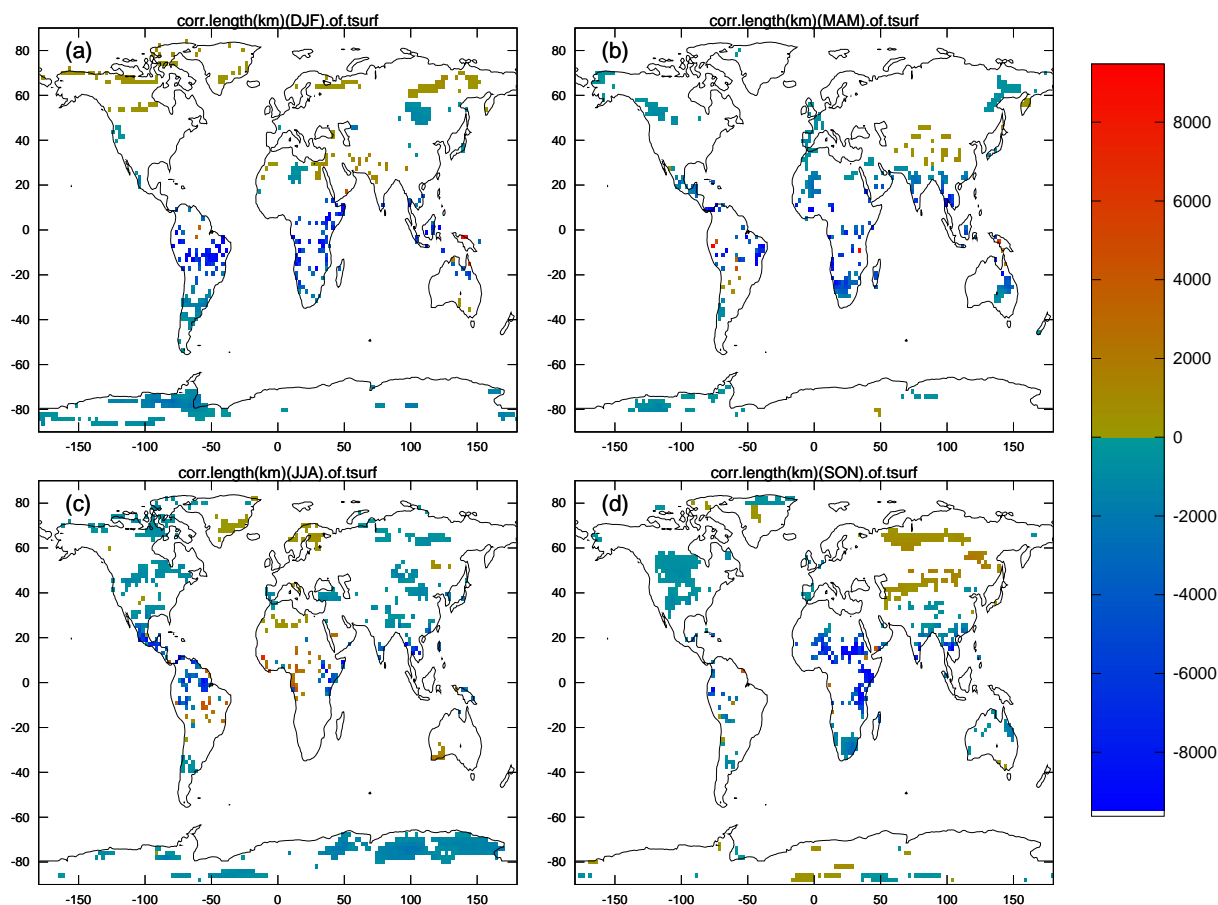
Fig. 9. Change in east-west correlation length scale for seasonal temperature (km) induced by soil moisture feedback. (a) DJF, (b) MAM, (c) JJA, (d) SON.
