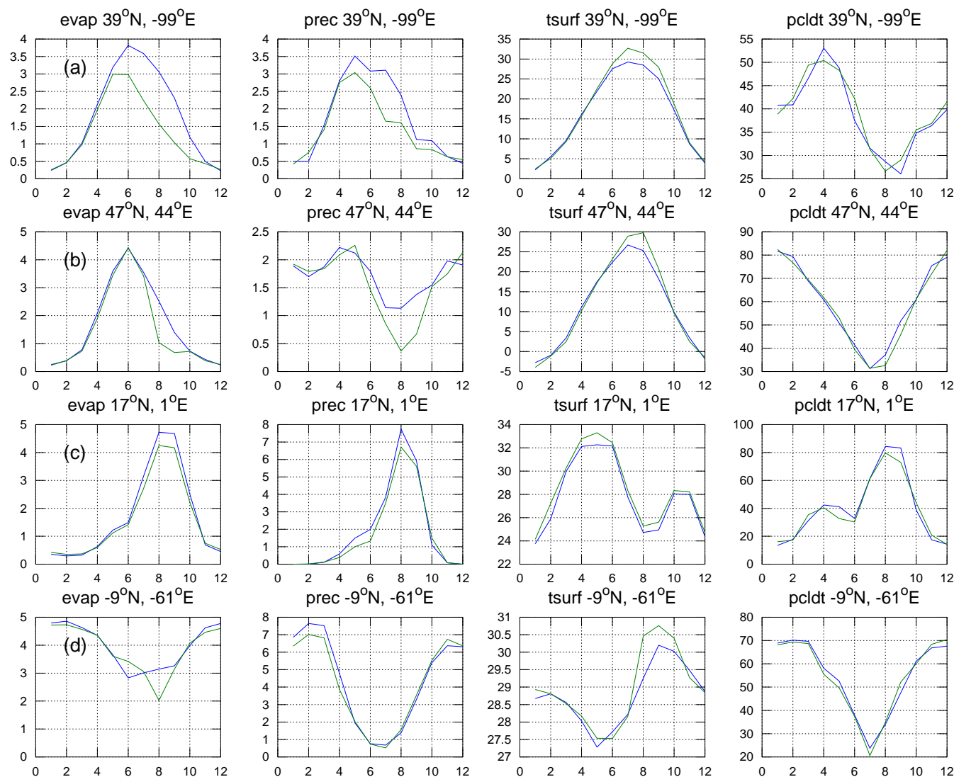
Fig. 5. Monthly mean climate for four representative grid points: (a) US Great Plains (39° N 99° W), (b) eastern Europe (47° N 44° E), (c) the Sahel (17° N 1° E), (d) the Amazon basin (9° S 61° W). From left to right, the columns show evaporation (mm/day), precipitation (mm/day), temperature (° C), and cloud fraction (%). Blue lines are for CLIM run, green lines DYNA run.
