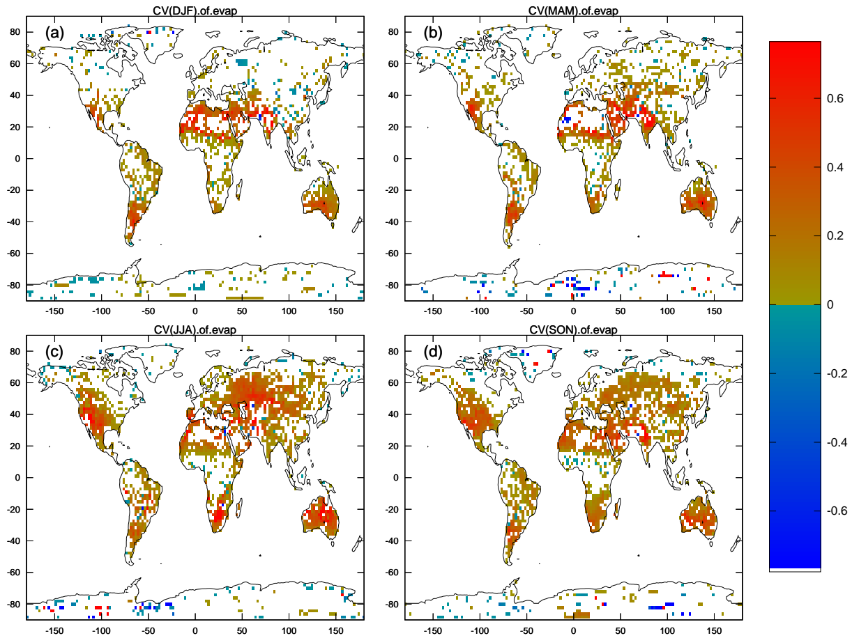
Fig. 6. Change in interannual coefficient of variation of seasonal evaporation (unitless) induced by soil moisture feedback (DYNA minus CLIM run). (a) DJF, (b) MAM, (c) JJA, (d) SON.
