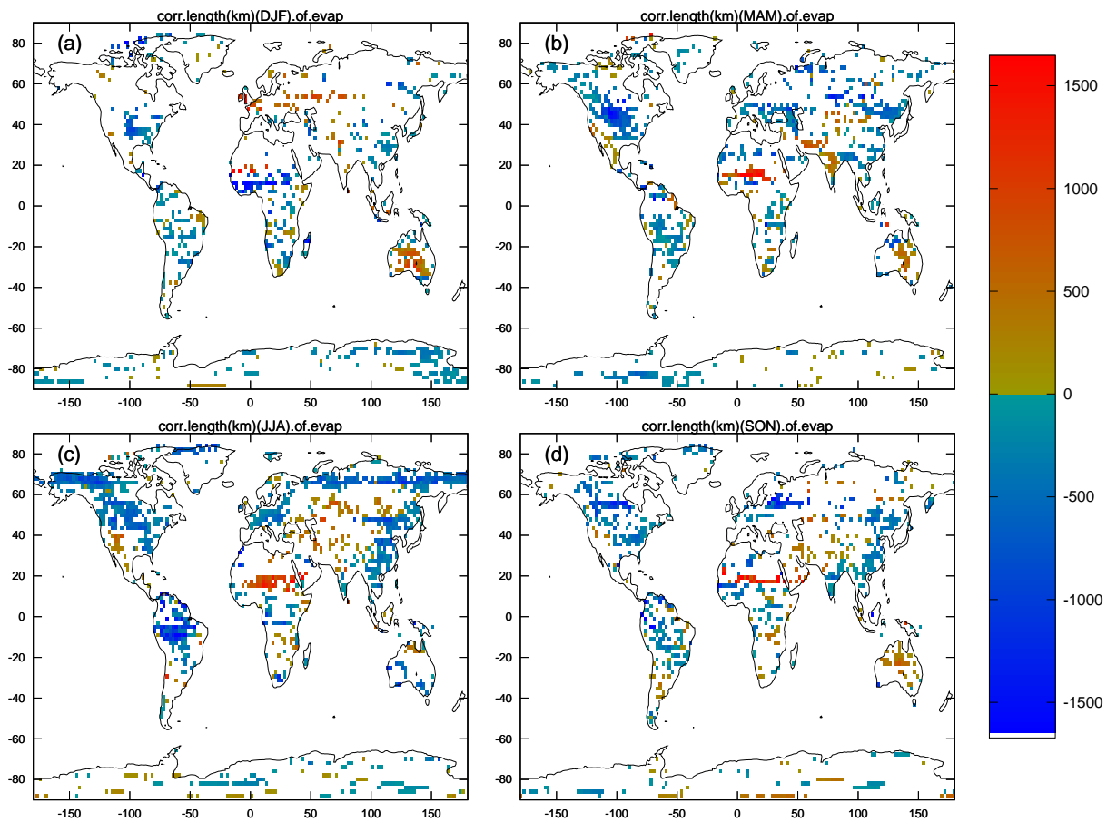
Fig. 8. Change in east-west correlation length scale for seasonal evaporation (km) induced by soil moisture feedback (DYNA minus CLIM run). (a) DJF, (b) MAM, (c) JJA, (d) SON.
