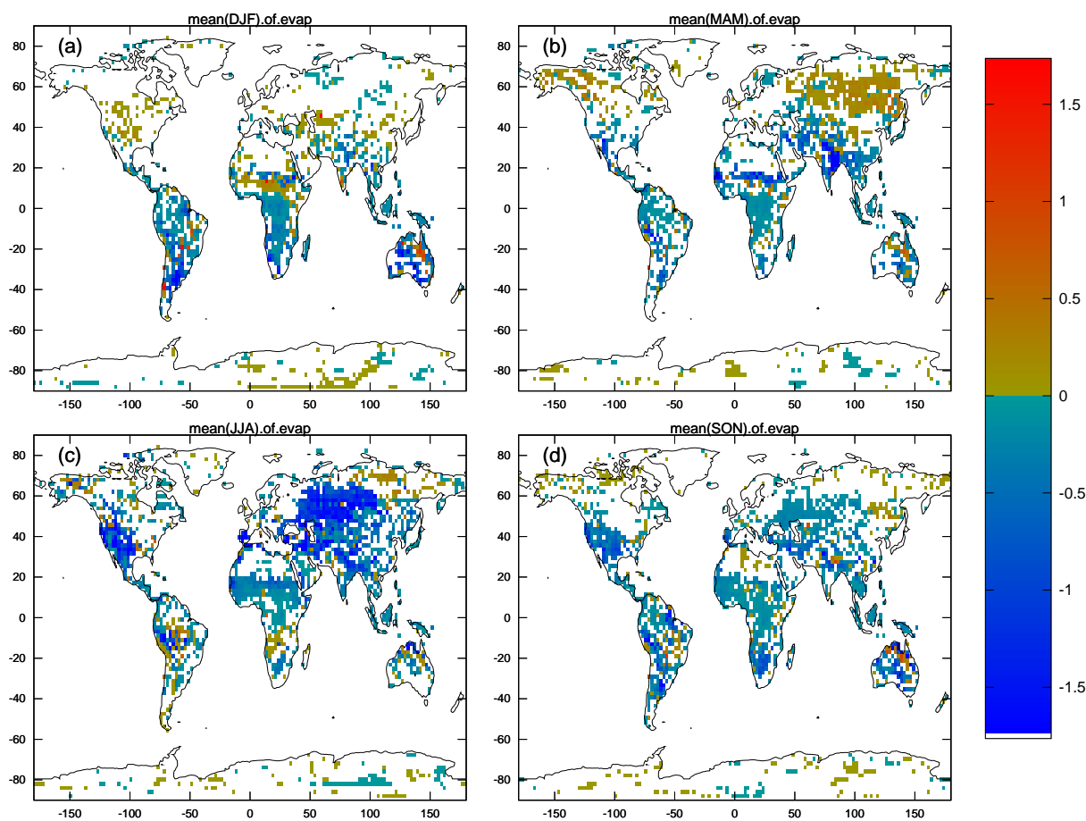
Fig. 1. Change in seasonal evaporation (mm/day) induced by soil moisture feedback (DYNA minus CLIM run). (a) December-January-February (DJF), (b) March-April-May (MAM), (c) June-July-August (JJA), (d) September-October-November (SON). In this and subsequent figures, increases are shown as orange to red, decreases as green to blue; only changes that are over land and are significant at the 0.1 level are shown.
