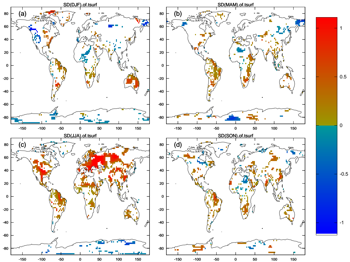
Fig. 7. Change in interannual standard deviation of seasonal temperature (K) induced by soil moisture feedback (DYNA minus CLIM run). (a) DJF, (b) MAM, (c) JJA, (d) SON.
