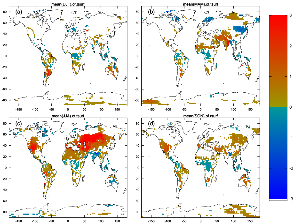
Fig. 3. Change in seasonal surface air temperature (K) induced by soil moisture feedback (DYNA minus CLIM run). (a) DJF, (b) MAM, (c) JJA, (d) SON.
