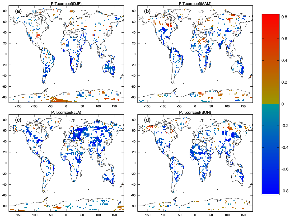
Fig. 10. Change in correlation coefficient between seasonal temperature and precipitation (dimensionless) induced by soil moisture feedback (DYNA minus CLIM run). Negative values mean that the correlation coefficient ( r ) became more negative, not that the strength of the correlation ( r^2 ) was reduced. (a) DJF, (b) MAM, (c) JJA, (d) SON.
