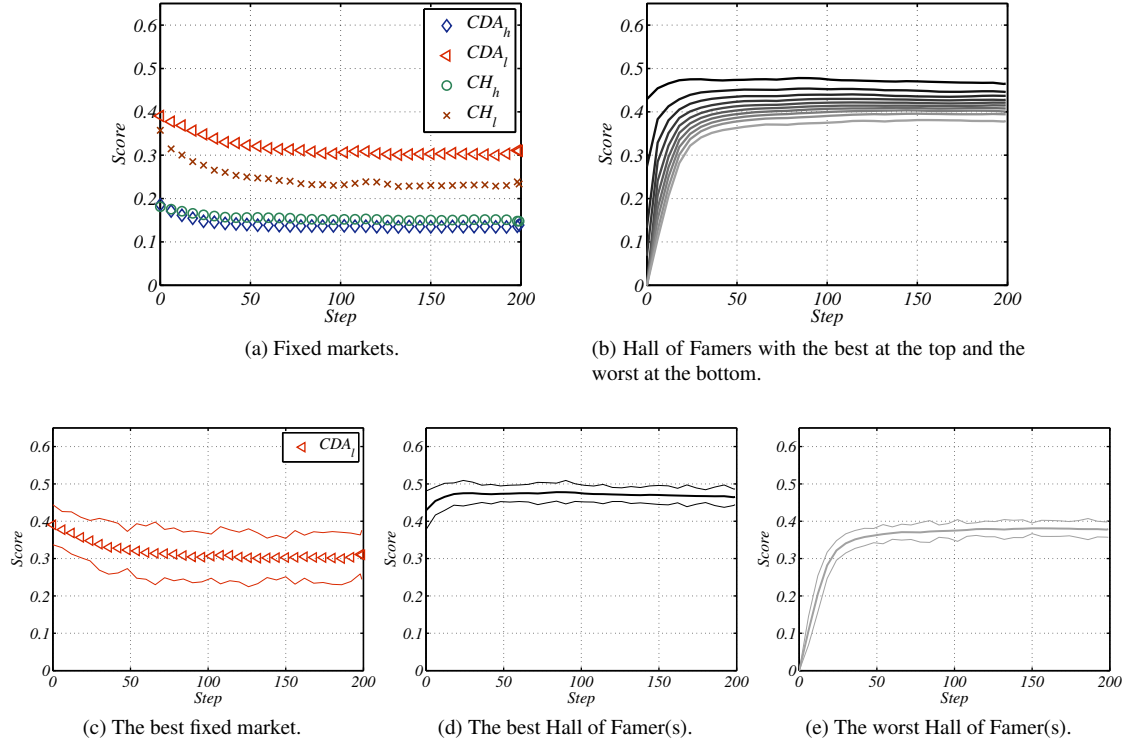
Figure 2: Scores of market mechanisms in the first set of grey-box experiments across 200 steps, averaged over 40 runs.
