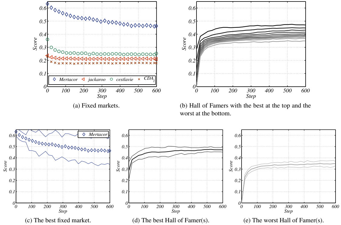
Figure 4: Scores of market mechanisms in the second set of grey-box experiments across 600 steps, averaged over 30 iterations.
