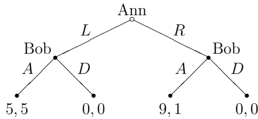
Figure 15: Extensive form representation of an ultimatum game where Ann either offers a fair (L) or unfair (R) proposal and Bob can accept (A) or reject (D).
